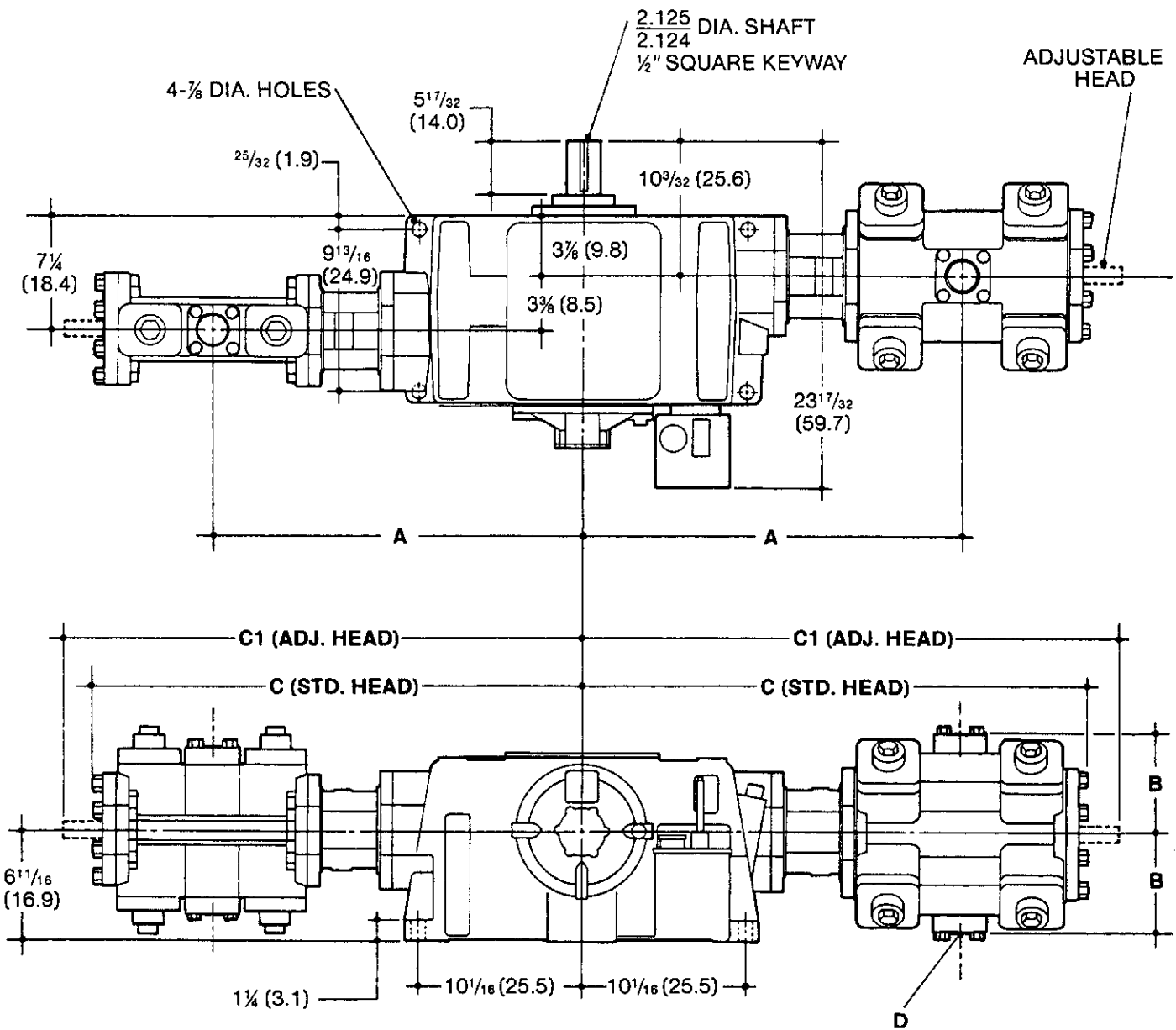
ALL DIMENSIONS IN INCHES (CM)
