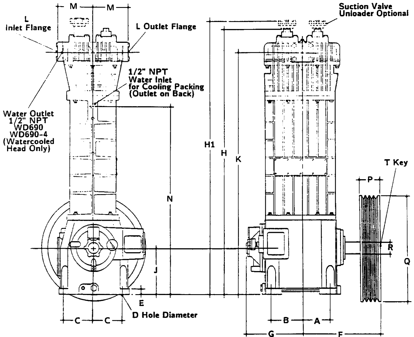
DIMENSIONS IN INCHES (CENTIMETERS)
