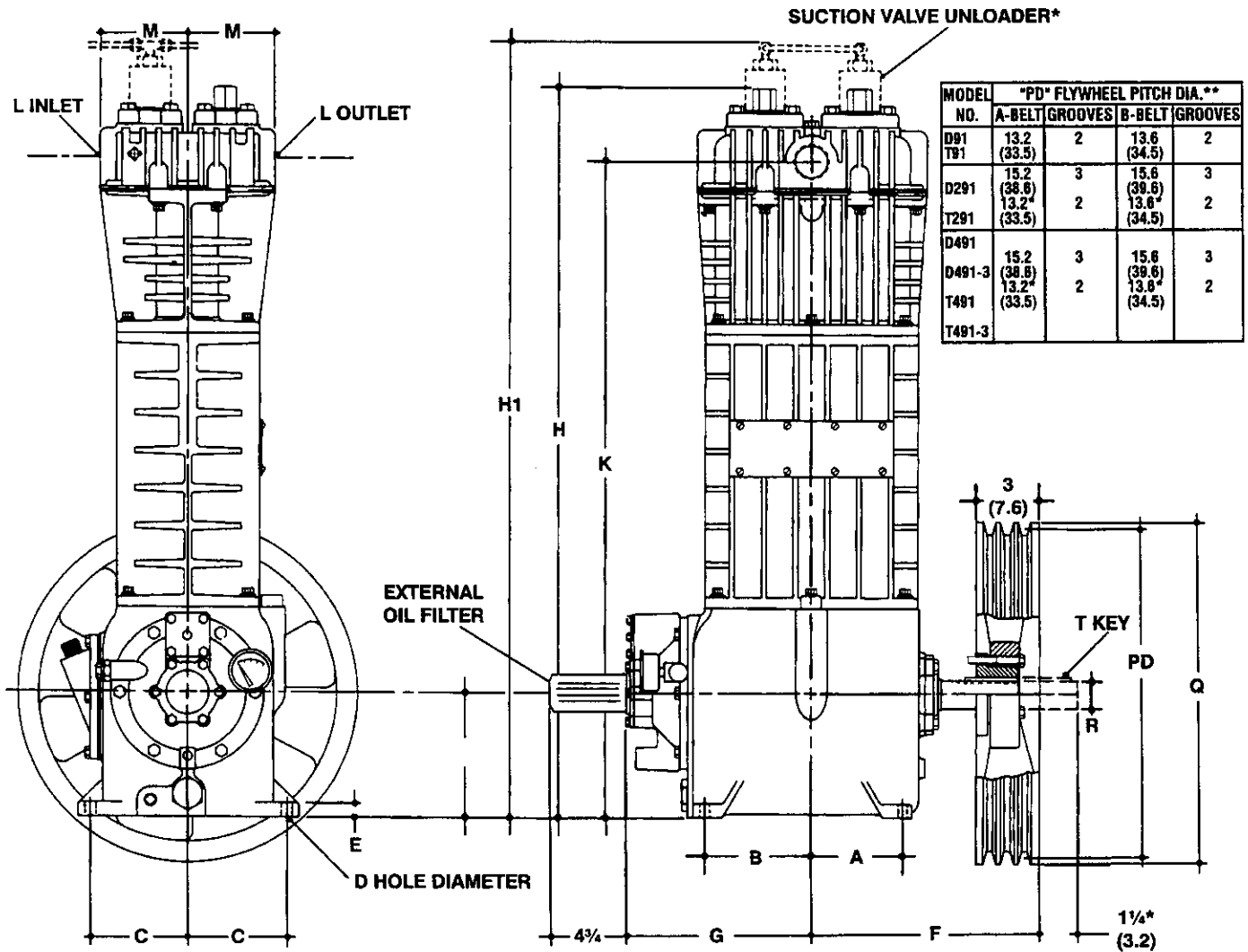
DIMENSIONS IN INCHES (CENTIMETERS)
