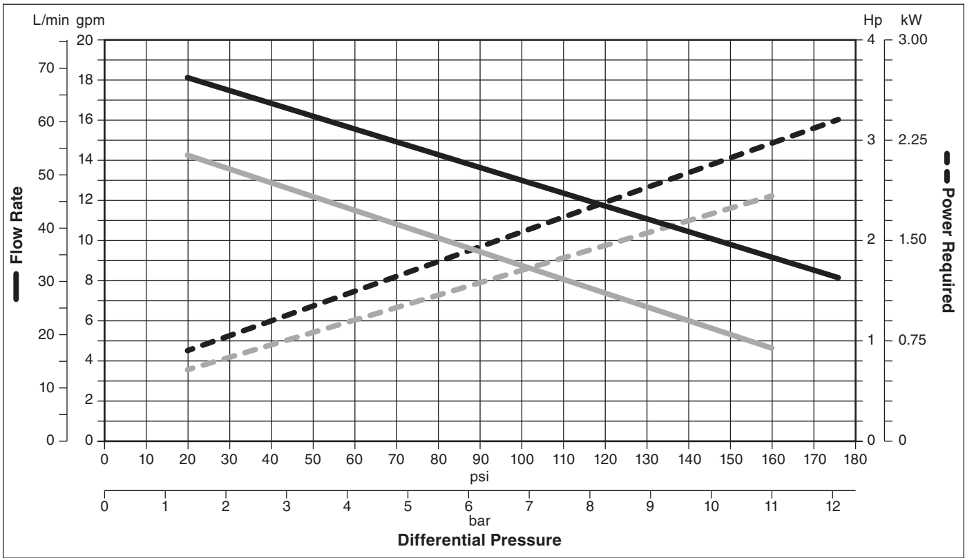
Model 16 Performance Curves 1
